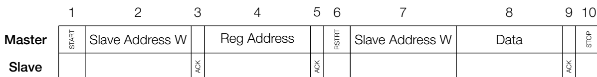
Figure 173: I 2 C Write Operation
