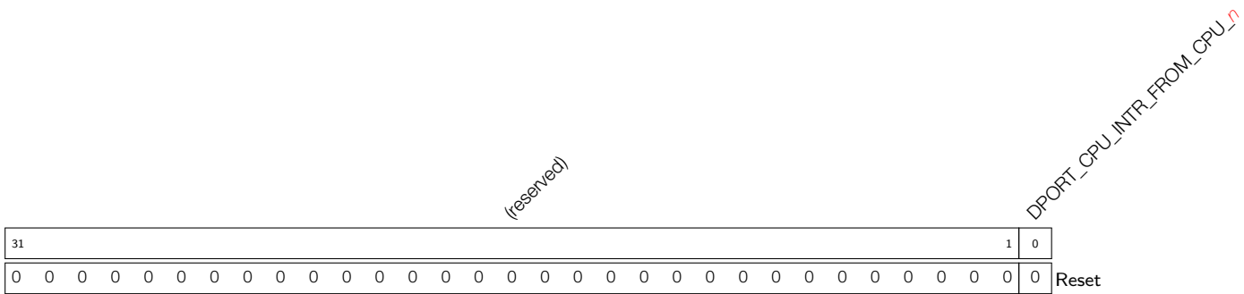
Register 5.21: DPORT_CPU_INTR_FROM_CPU_n_REG (n: 0-3) (0xDC+4*n)
