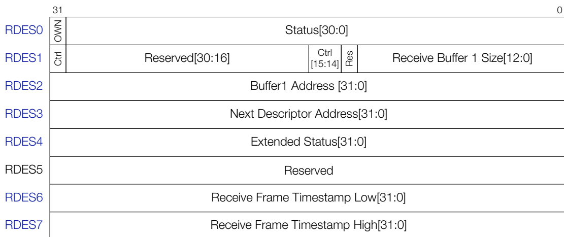
Figure 50: Receive Descriptor
