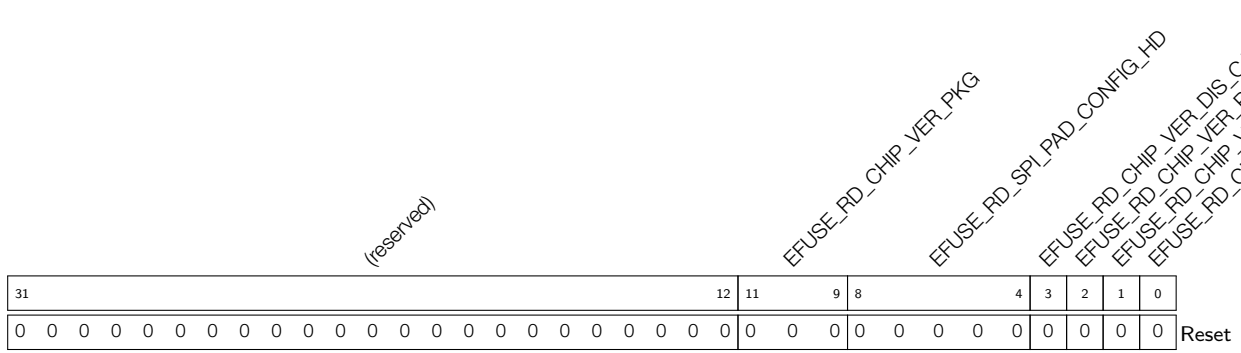
Register 20.4: EFUSE_BLK0_RDATA3_REG (0x00c)
