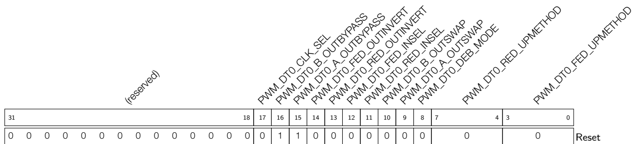
Register 16.23: PWM_DT0_CFG_REG (0x0058)
