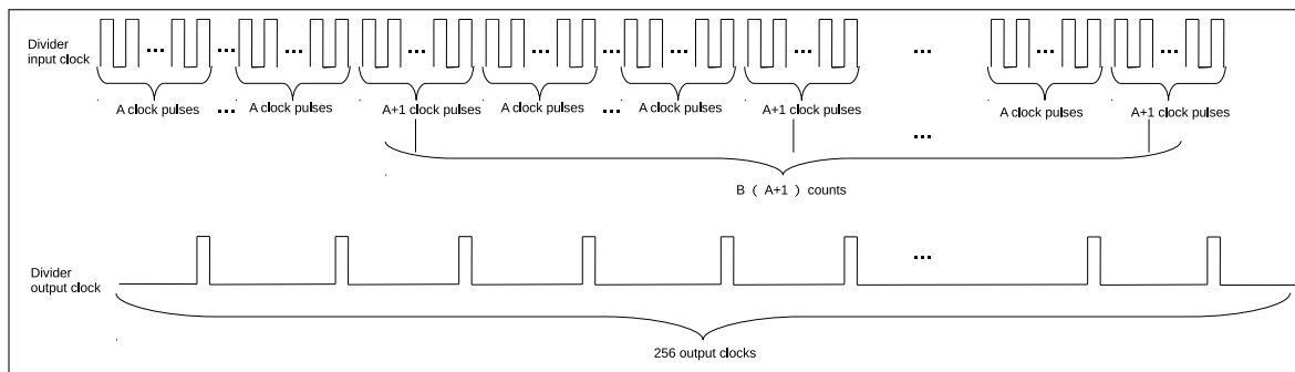
Figure 89: LED_PWM Divider
