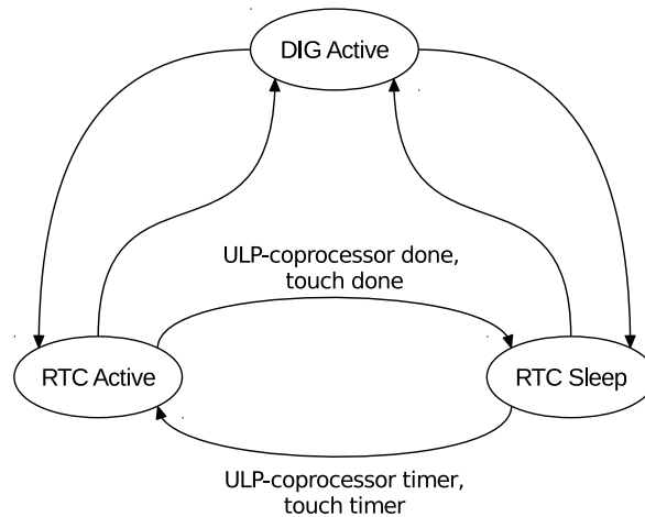
Figure 182: RTC States
