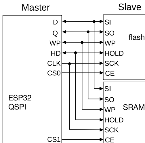
Figure 20: Parallel QSPI
