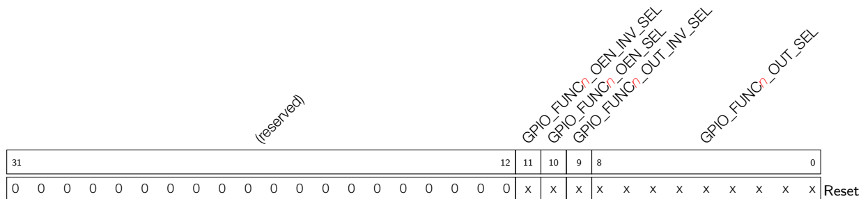
Register 4.32: GPIO_FUNC n _OUT_SEL_CFG_REG ( n : 0-19, 21-23, 25-27, 32-33) (0x530+0x4* n )
