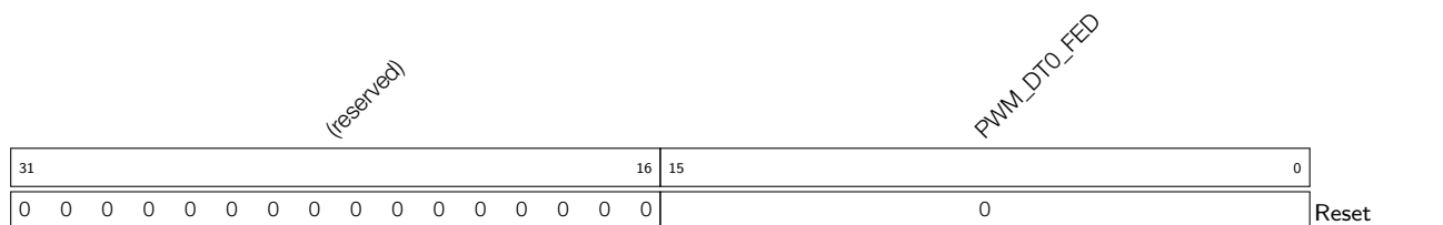
Register 16.24: PWM_DT0_FED_CFG_REG (0x005c)
