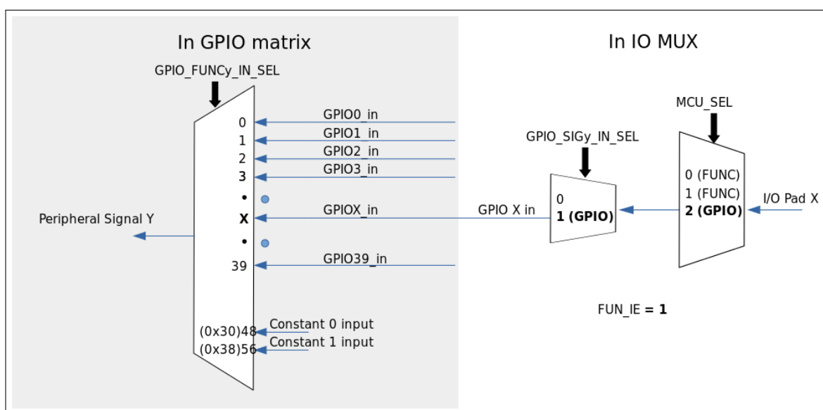
Figure 8: Peripheral Input via IO_MUX, GPIO Matrix
