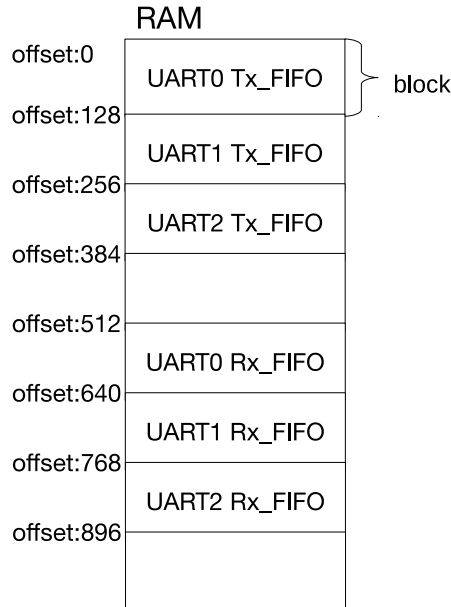
Figure 83: UART Shared RAM
