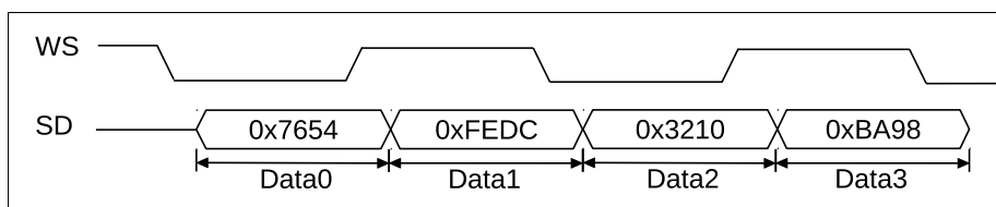
Figure 69: The First Stage of Receiving Data
