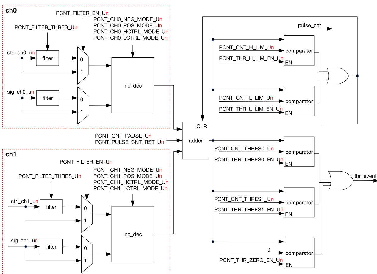
Figure 123: PULSE_CNT Architecture
