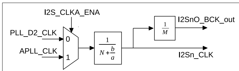
Figure 64: I2S Clock
