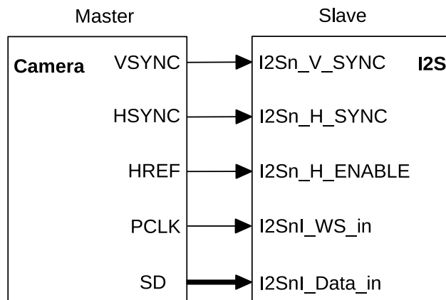
Figure 78: Camera Slave Receiving Mode
